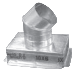
No.3500FA R4.2 w/flange No.3500NFA R4.2 w/no flange No.3600FA R6.0 w/flange No.3600NFA R6.0 no flange No.3600FA8 R8.0 w/flange No.3600NFA8 R8.0 no flange Insulated Metal Top Register Box Angle Outlet
